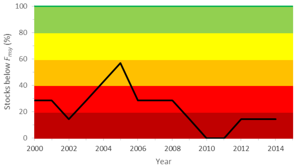
Figure 123. Percentage of stocks where fishing pressure is at or below the maximum sustainable level ( F_{msy} ) for 7 stocks in the Black Sea (black curve). The colors indicate visually the compliance with the goals of the Common Fisheries Policy, where all stocks (100%) shall be fished at or below F_{msy} in 2015, latest in 2020. In 2014, only one stock (Black Sea sprat, Spr_{BS} , 14%) fulfilled that requirement. [BlackSea_Oct14_16.xlsx]
