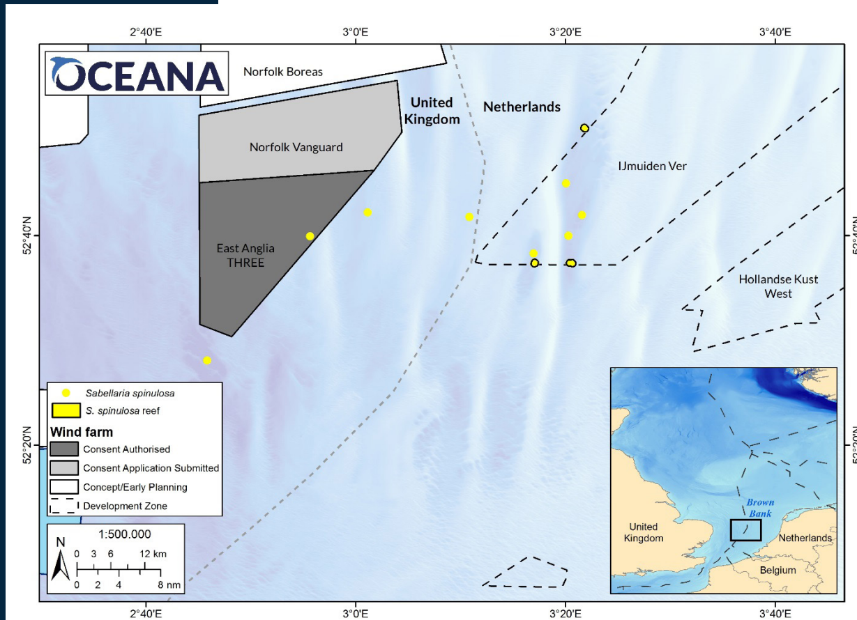
Figure 18. Locations of newly discovered Sabellaria spinulosa reefs, and other observations of S. spinulosa , in relation to planned wind farms in the Brown Bank area.
