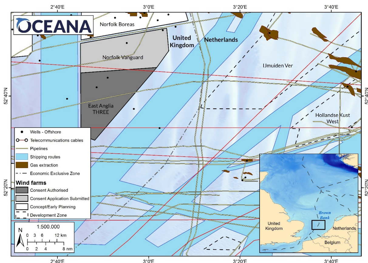
Figure 4. Shipping lanes and major offshore infrastructure in Brown Bank, including cables, pipelines, gas extraction areas, and wind farms (both authorised and potential projects).
