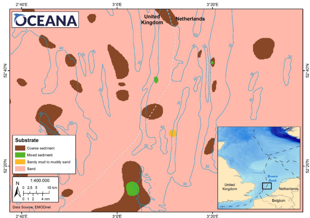
Figure 2. Substrate types and bathymetry of Brown Bank.
