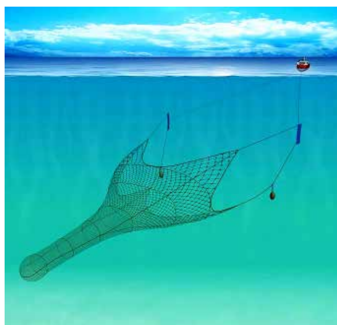
Figure 13. Semi-pelagic otter trawl, where the doors are lifted off the seabed while the ground gear remains in contact with the seafloor (top). Midwater or pelagic trawl where none of the gear is touching the seabed. The doors in both types of trawls have a higher height aspect ratio when compared to bottom otter trawls to generate the necessary lift (bottom).
